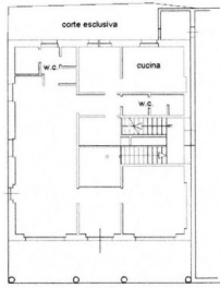
PIANO TERRA h = 3.10 m
